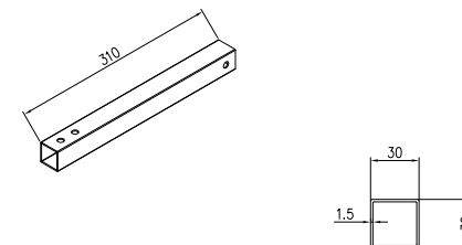
Telescopic rod-A × 2
