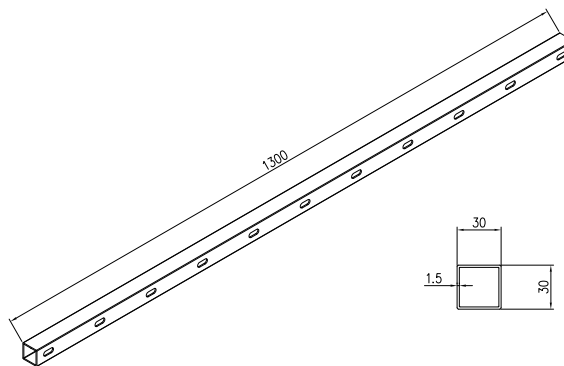
Cross arm × 1
