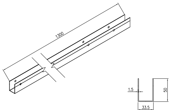
Main post × 2
