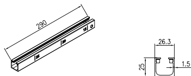
Telescopic rod-B × 2
