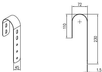
Hook × 2
