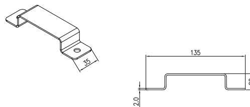
Hook × 2
