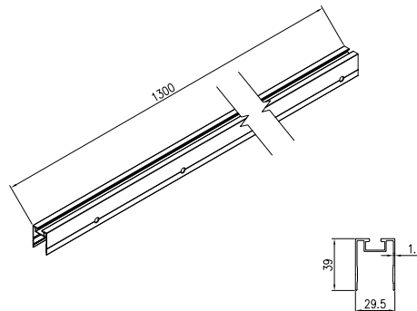
Sub post × 2
